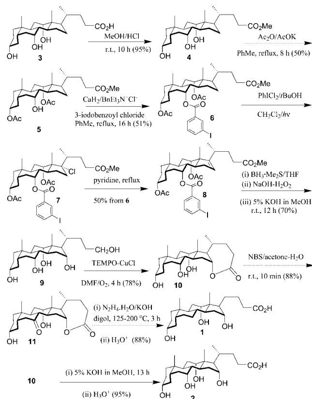
Scheme 1. Synthesis of 1 and 2 from cholic acid.
