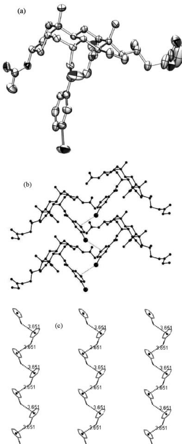
Figure 2. (a) ORTEP diagram of single-crystal X-ray structure; (b) GS view of C–iodine \cdots Ar interactions (c) Packing pattern of 3-iodoaryl moiety of compound 6 using mercury 1.4.1.
