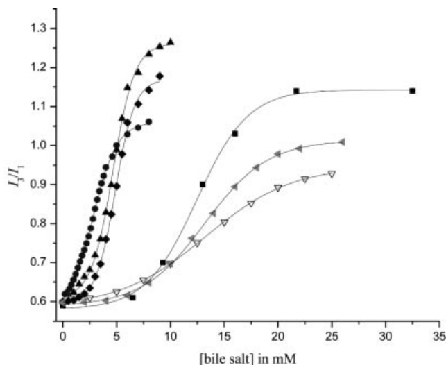
Figure 4. The ratio of vibronic bands ( I_3/I_1 ) of pyrene fluorescence as a function of bile salt concentration. Concentration of pyrene was ca. 1 \mu\text{M} in tris buffer at pH 9. Pythocholate (black circles), deoxycholate (black triangles), chenodeoxycholate (black diamonds), cholate (open triangles), 16\alpha -hydroxycholate (grey triangles), avicholate (black squares).
