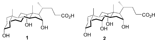
Figure 1. Pythocholic acid (1) and 16 \alpha -hydroxycholeic acid (2).
