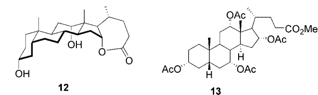
Figure 3. Pythocholic lactone and methyl 3a,7a,12a,16a-tetraacetoxo-5 \beta -cholan-24-oate.
